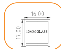
DL16 10mm
